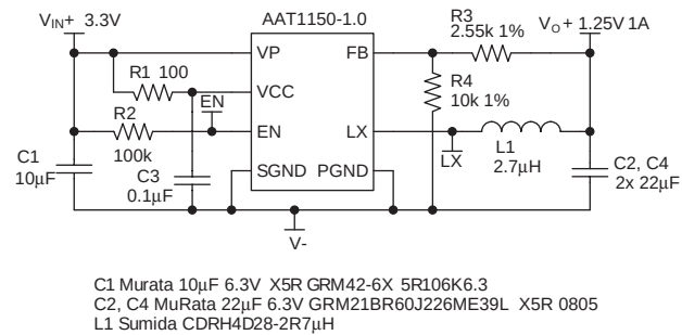
Figure 6: 3.3V to 1.25V Converter (Adjustable Output).
